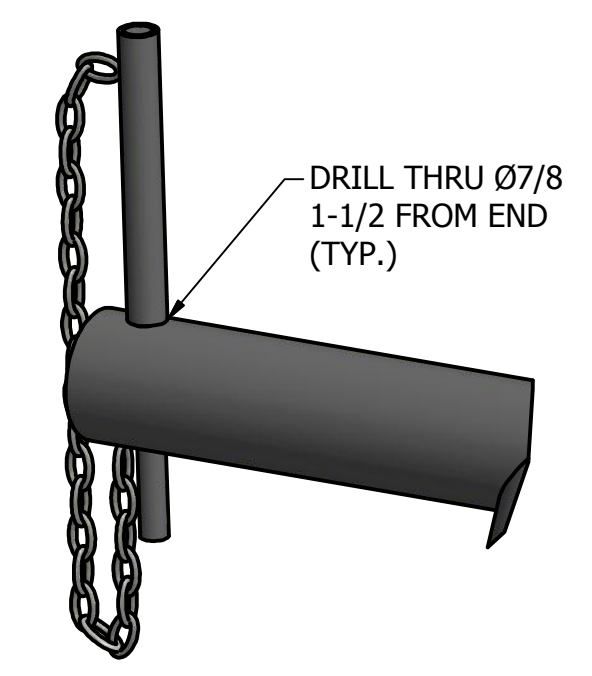
DETAIL A
