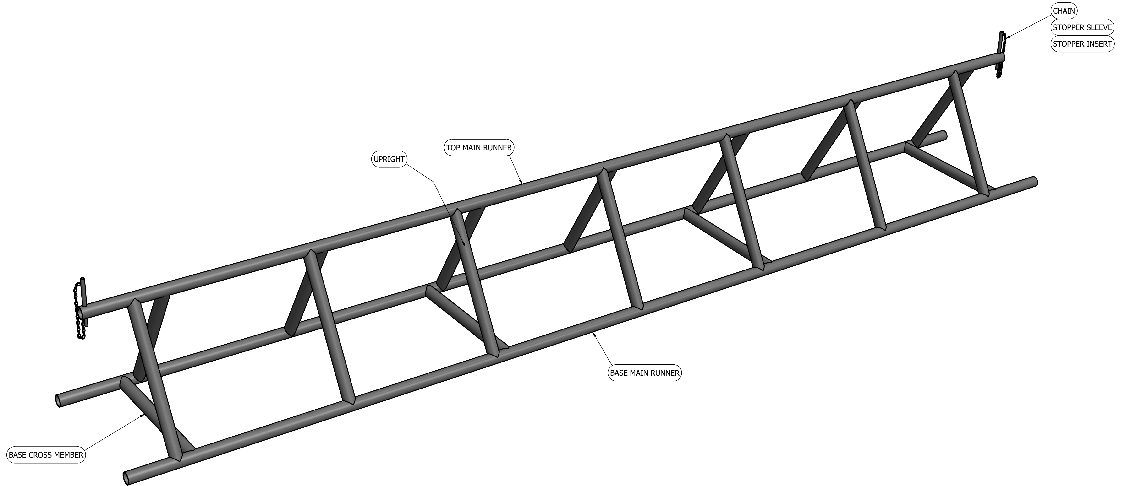
ISOMERIC VIEW OF 28' PIPE RACK
