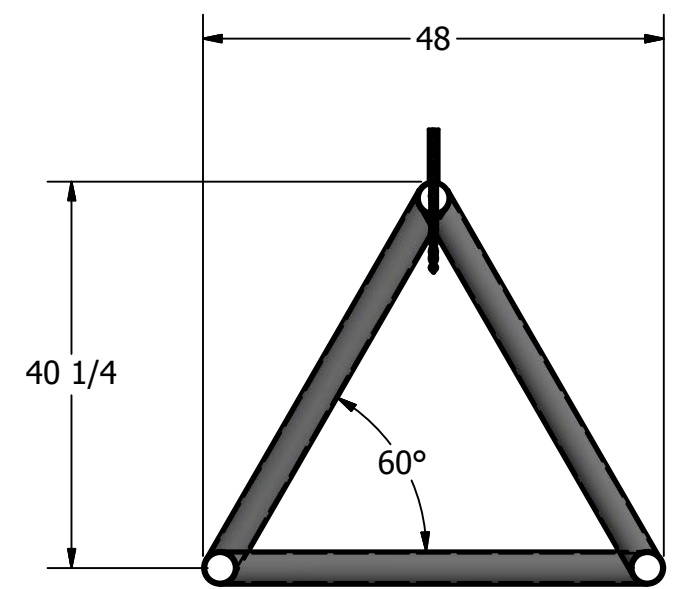
VIEW B-B
